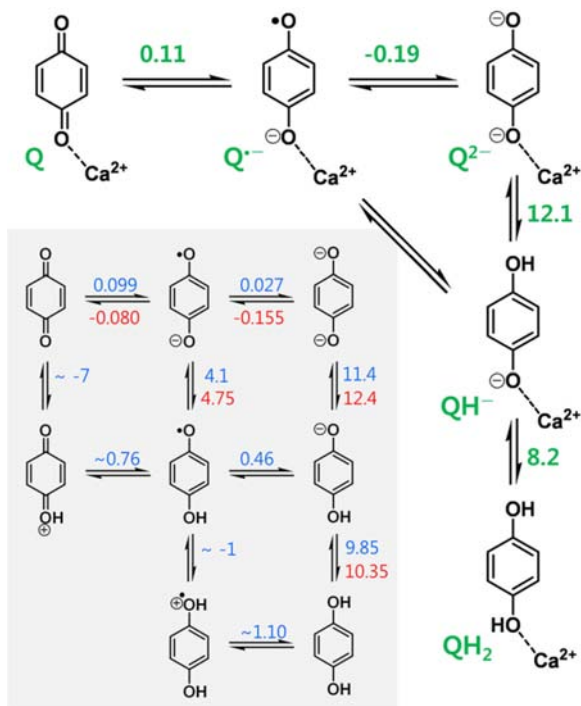
Scheme 1. Partial Nine-Member Square Scheme for CaCTAQ Utilized in the Digital Simulation and Analogous Schemes for BQ and DMBQ 67
